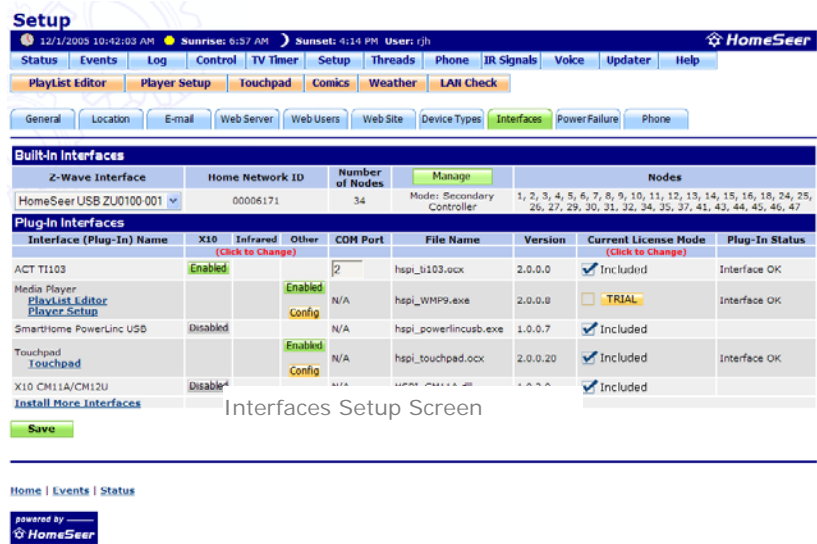
Figure 4: Interface Setup
